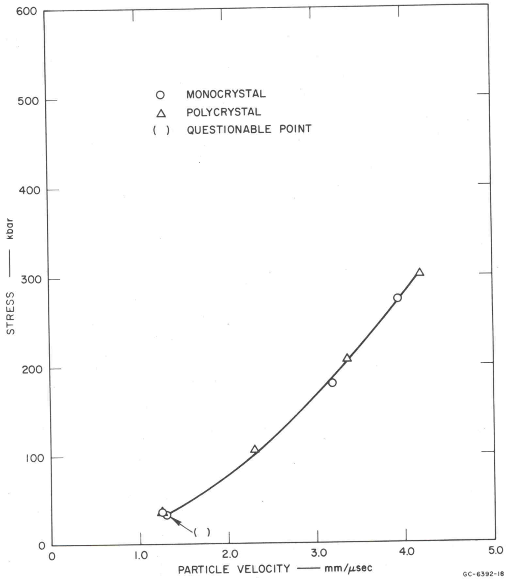
FIG. 18 HUGONIOT DATA FOR ICE ( \sigma - u )
