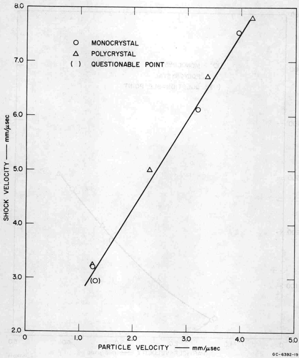
FIG. 19 HUGONIOT DATA FOR ICE ( U - u )
